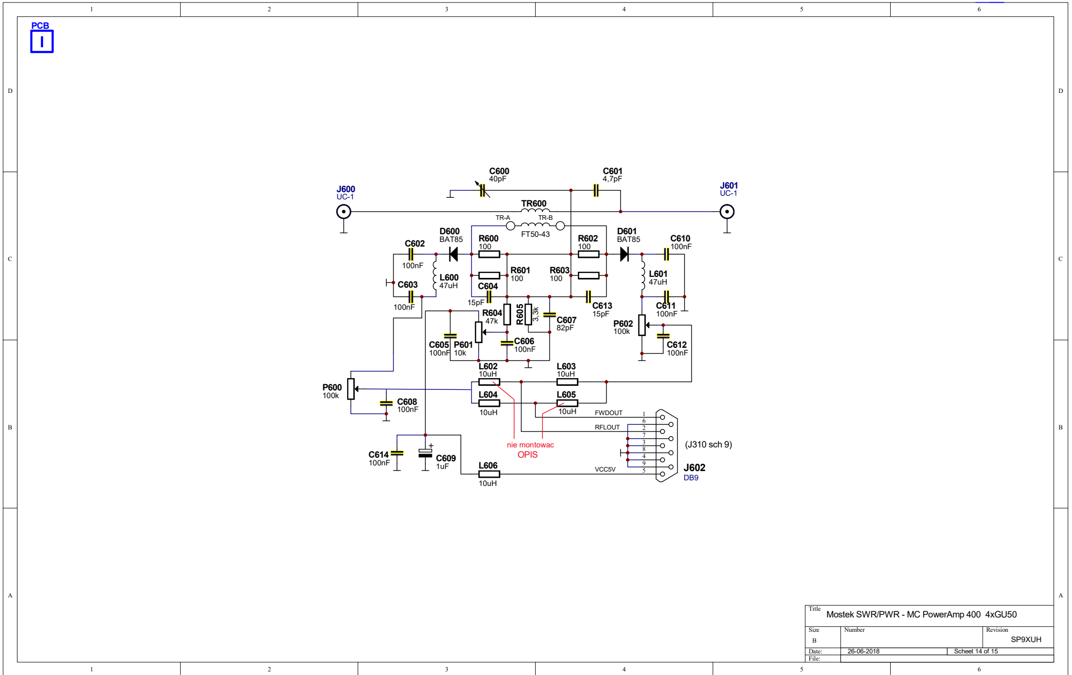
Schemat 14 - Mostek SWR/PWR.
